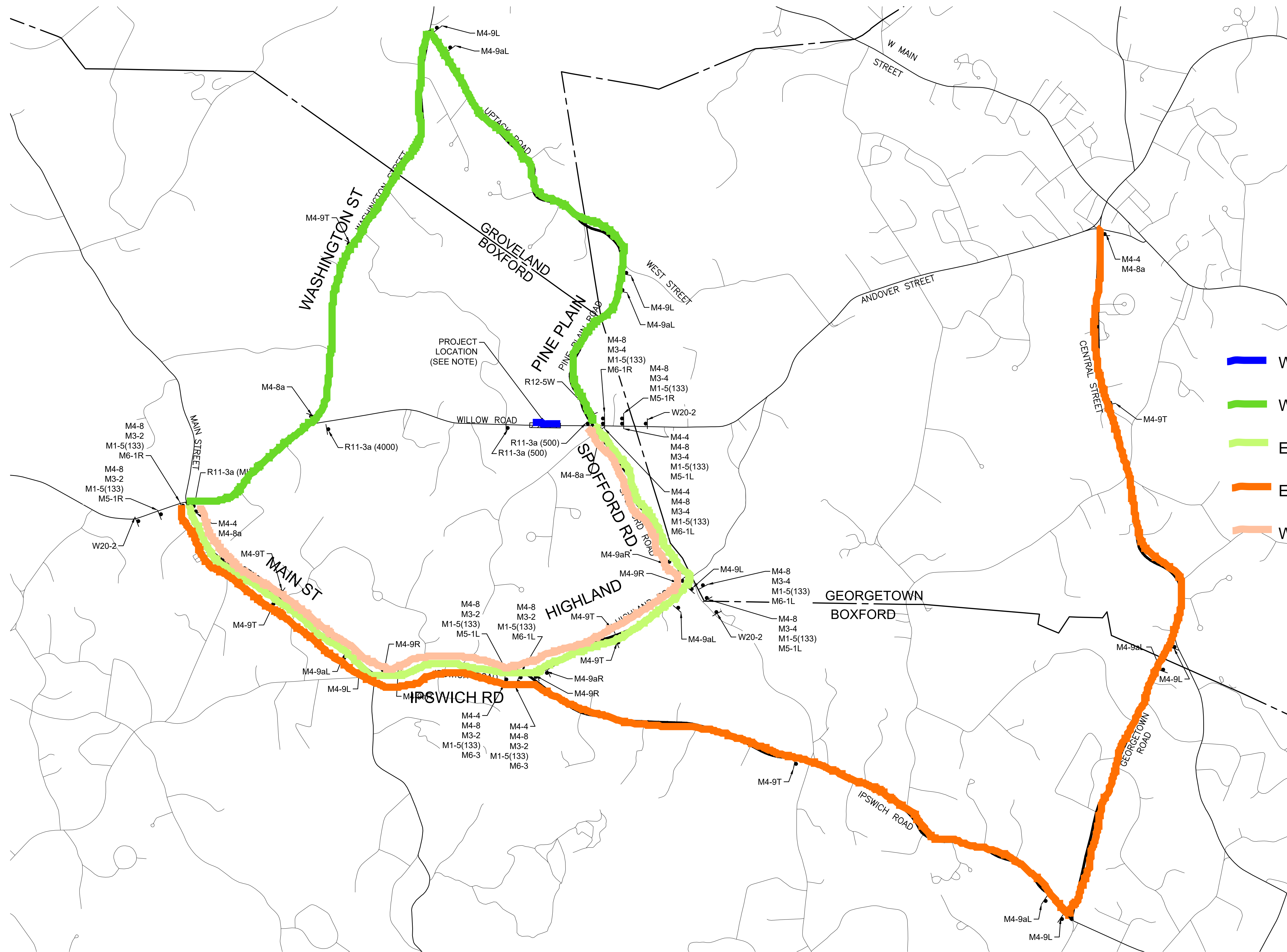
BRIDGE CLOSURE DETOUR PLAN SCALE: 1" = 750'
