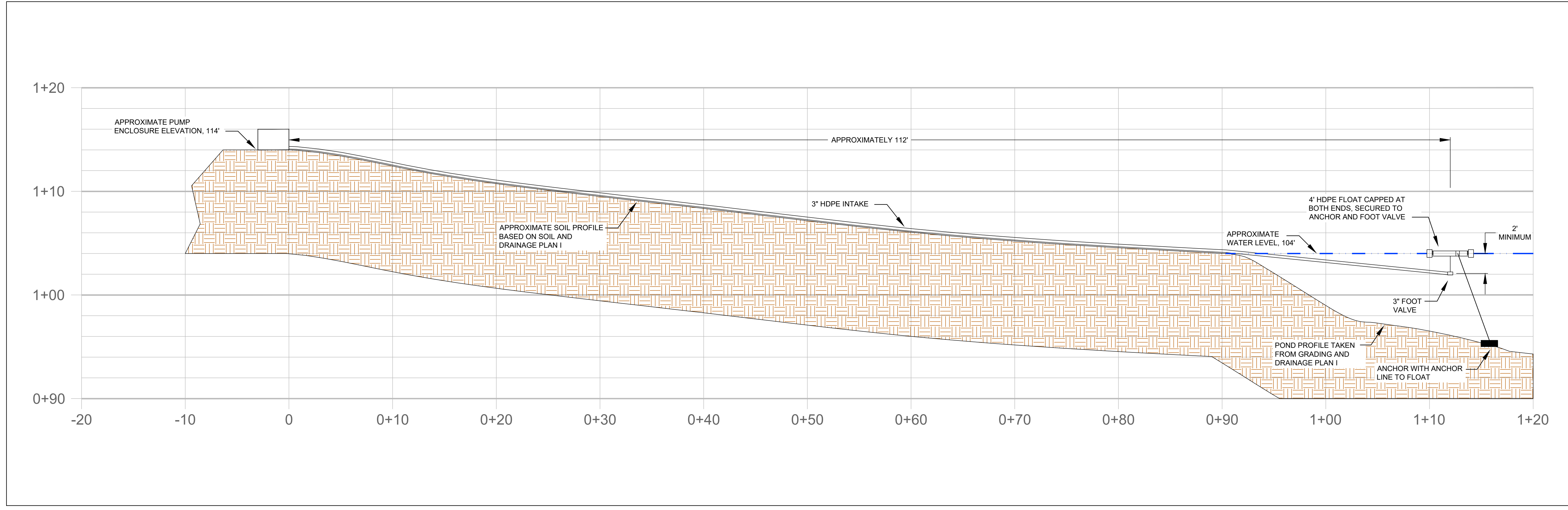
APPROXIMATE PUMP PROFILE 1" = 5'-0" P-1
