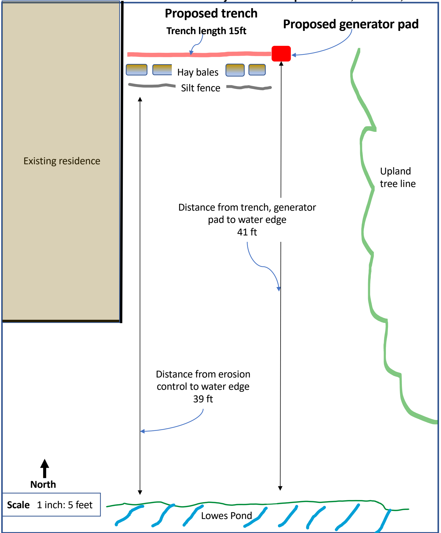
Attachment 2 - Detailed plan for proposed trench/generator pad for installation of full-house generator at Moore residence 112 Ipswich Rd Boxford, Mass
