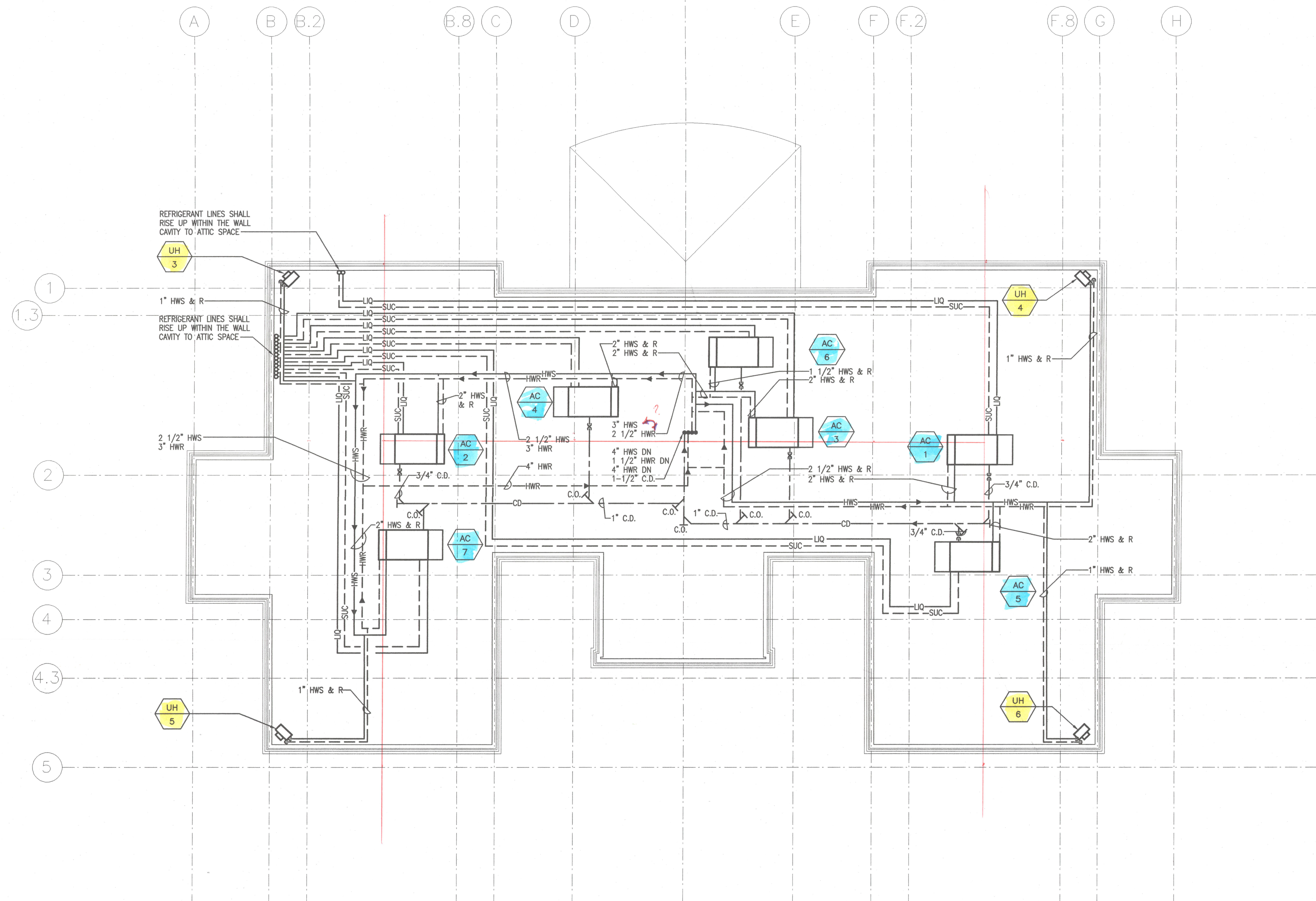
MECHANICAL ATTIC PIPING PLAN SCALE: 1/8"=1'-0"
