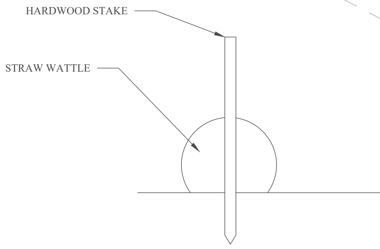
STRAW WATTLE DETAIL
