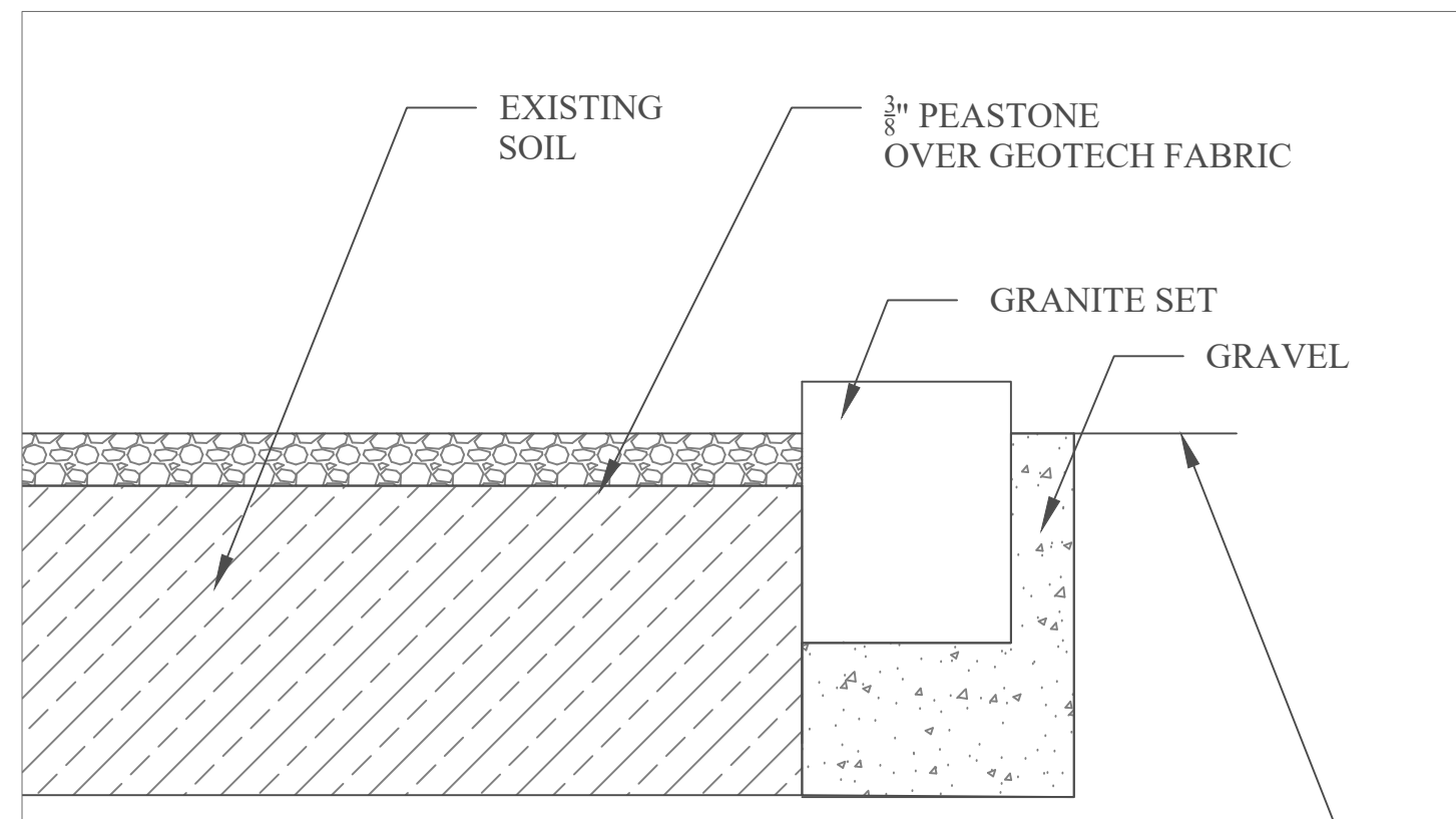
STONE/EDGING DETAIL
