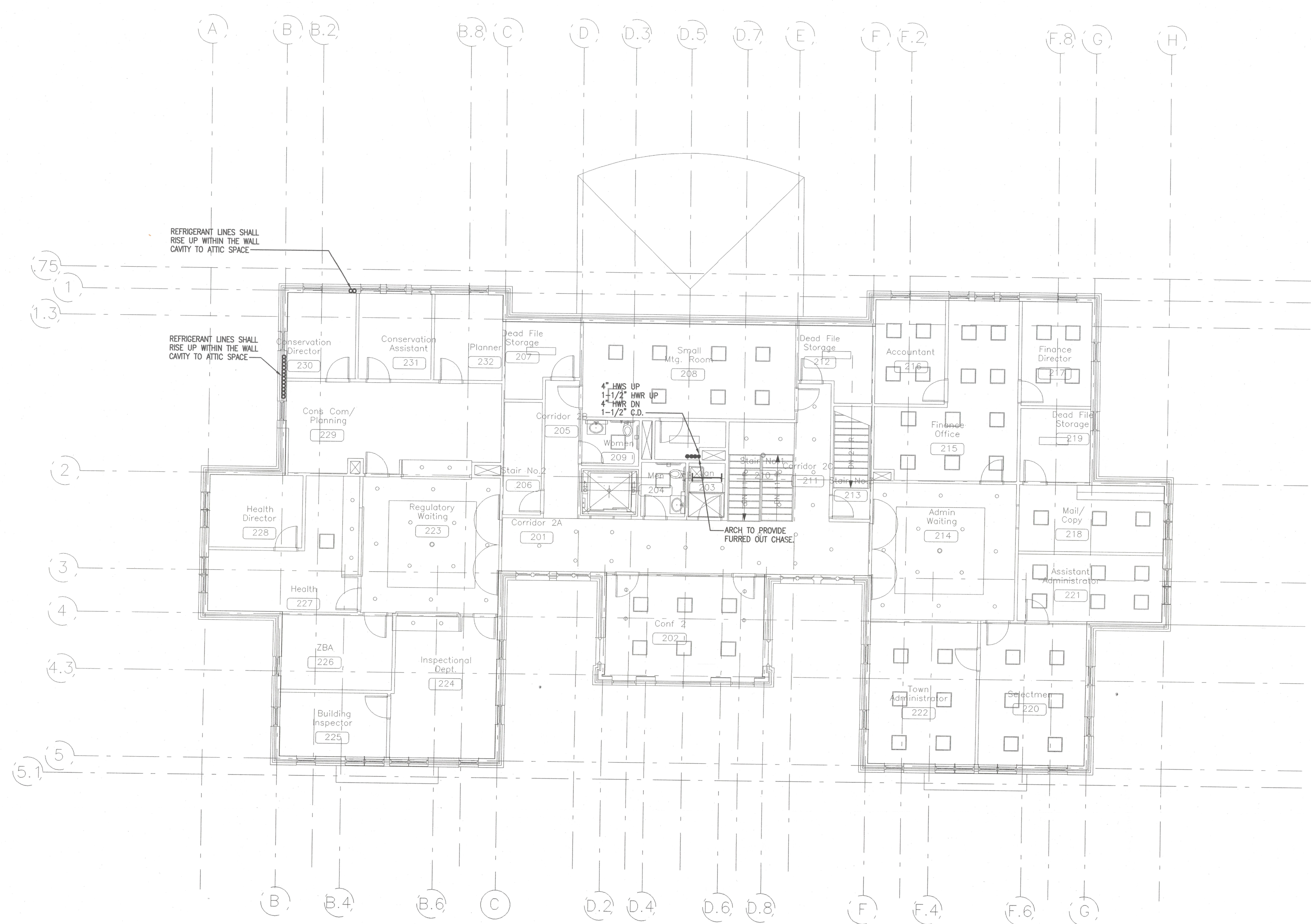
MECHANICAL SECOND FLOOR PIPING PLAN SCALE: 1/8"=1'-0"
